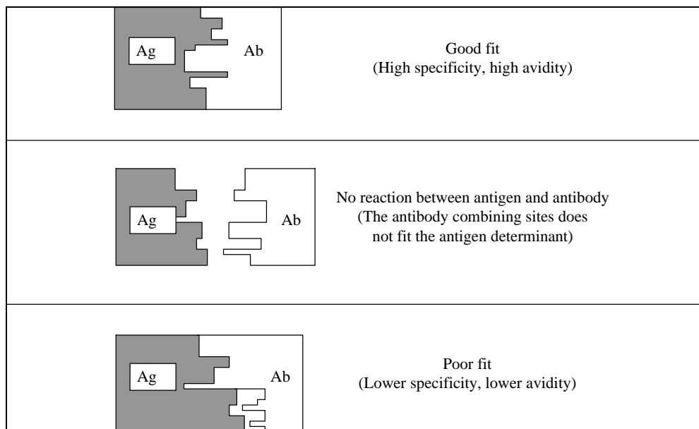
Figure 10: Antigen-antibody binding.
